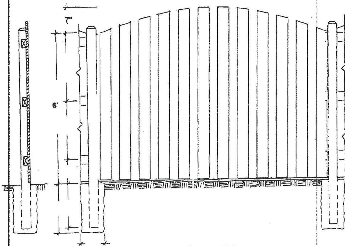
SIDE VIEW
